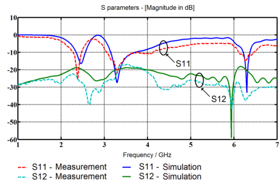
Figure 15. Measured and simulated results of S parameter of the proposed MIMO PIFA antenna.
