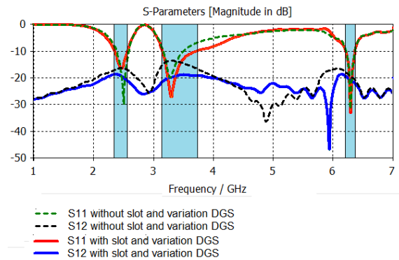
Figure 10. The S parameters of MIMO antenna with and without slot and variation DGS structures at the distance of 4 mm from edge to edge.
