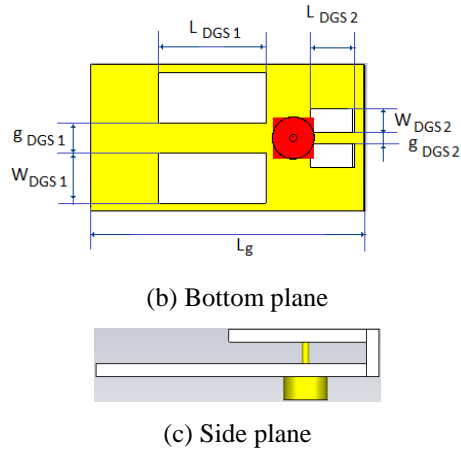
Figure 1. Structure of the proposed triple-band PIFA antenna.
